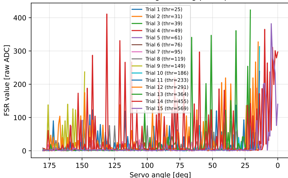
FSR raw value vs angle during press phase
